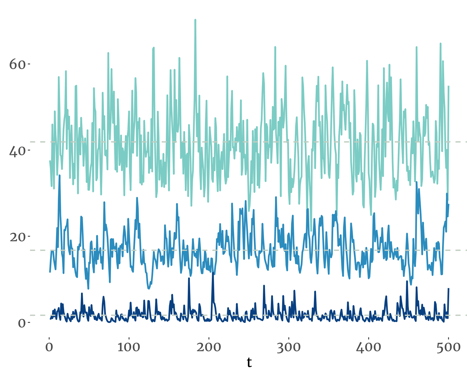
Time series
