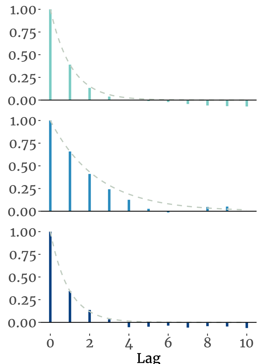
Sample ACF
