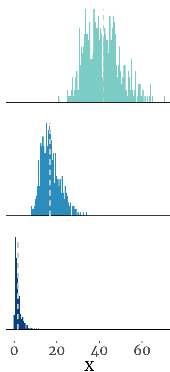
Marginal distribution
