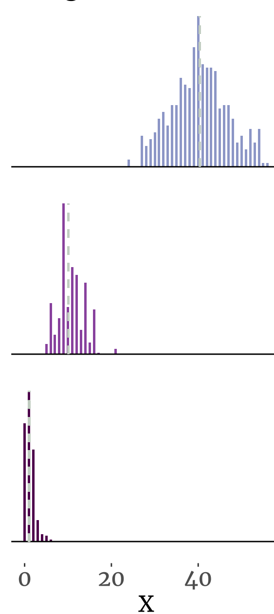
Marginal distribution
