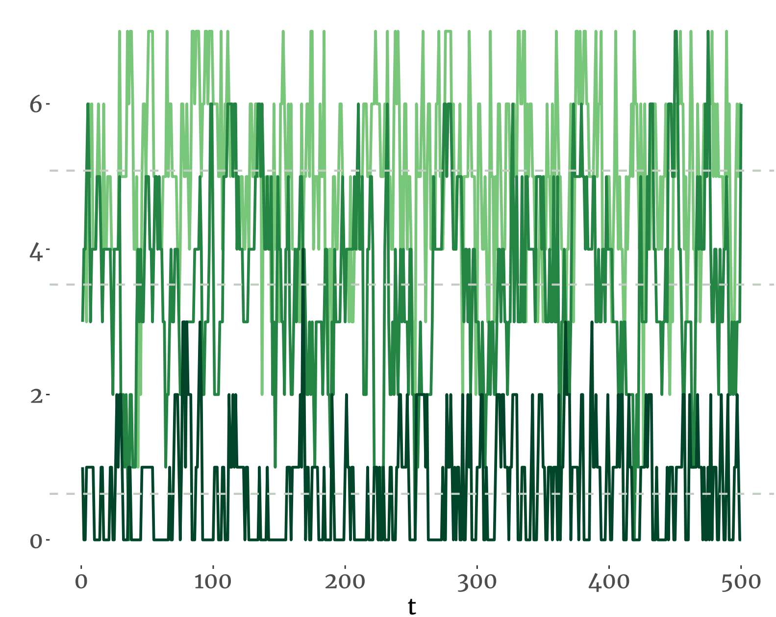
Time series
