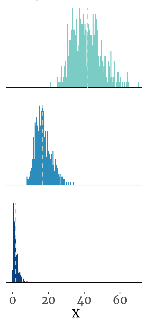
Marginal distribution
