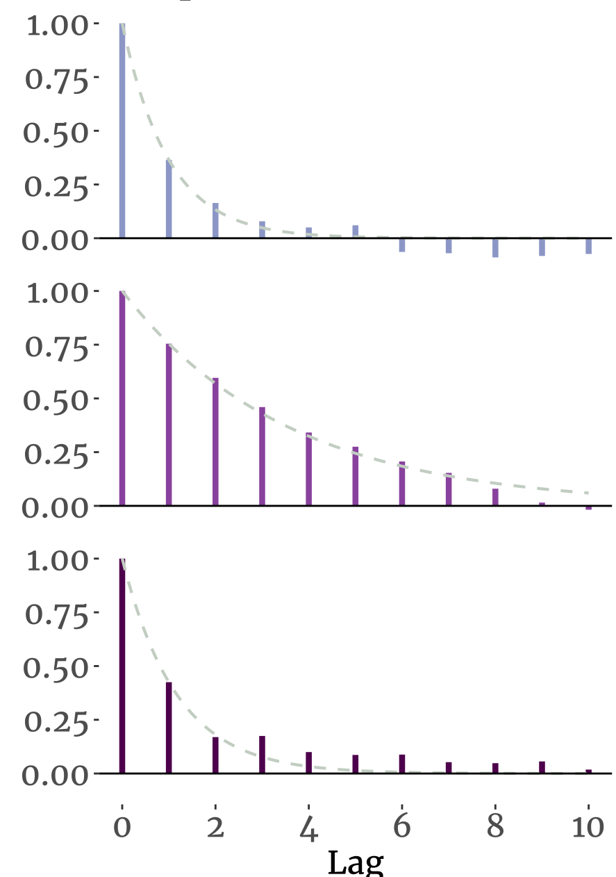
Sample ACF
