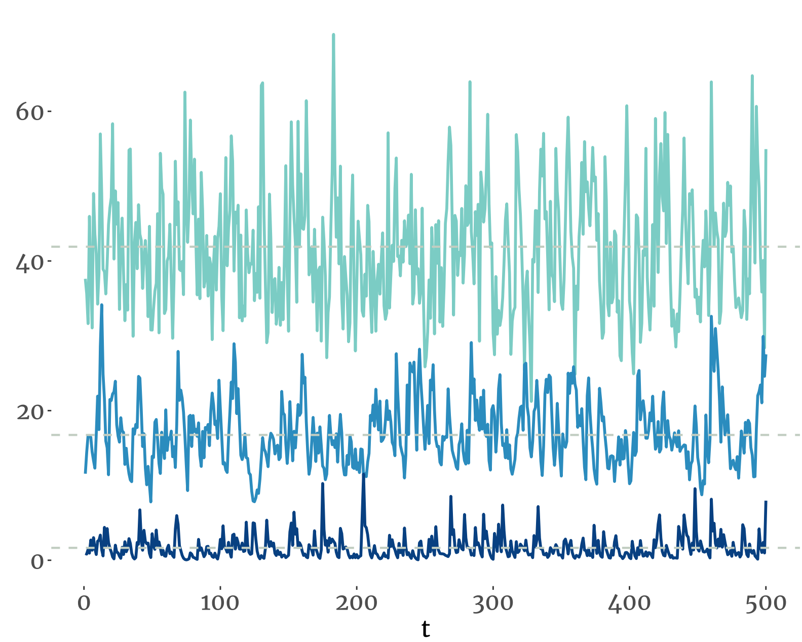
Time series
