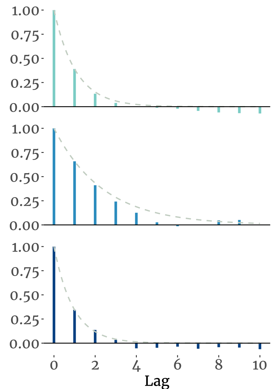
Sample ACF
