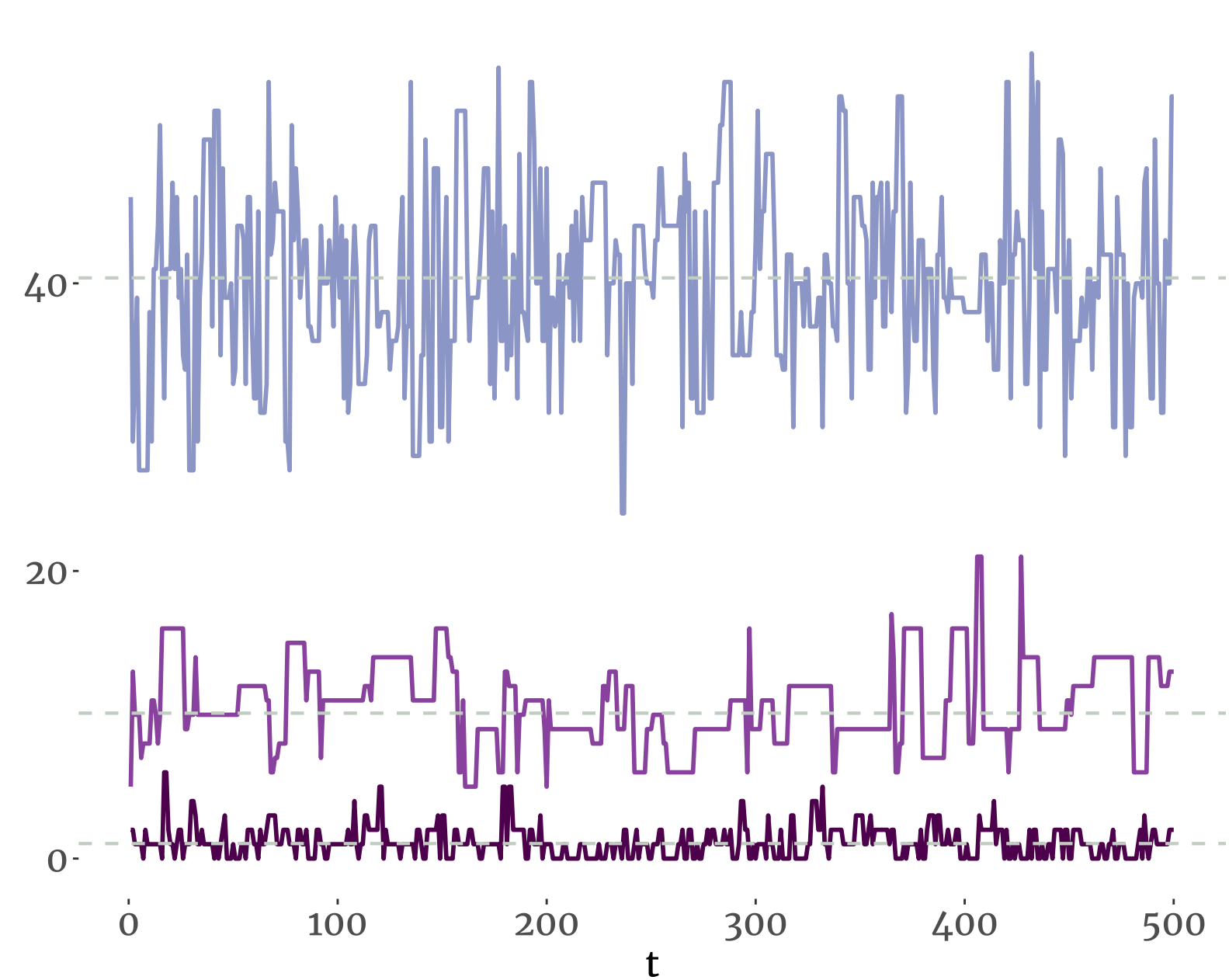
Time series
