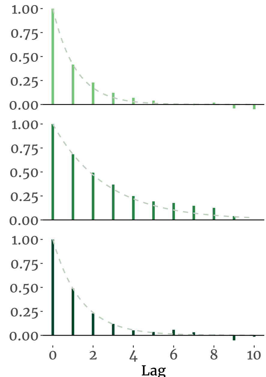
Sample ACF
